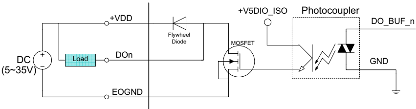
Figure 1-12: Isolated Digital Output Sample Application Circuit
