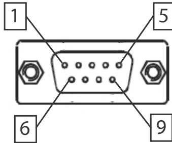
Figure 1-13: CAN Port
