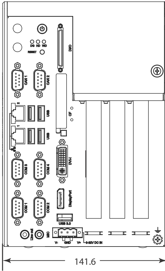
Figure 1-3: MXC-2300 Front View
