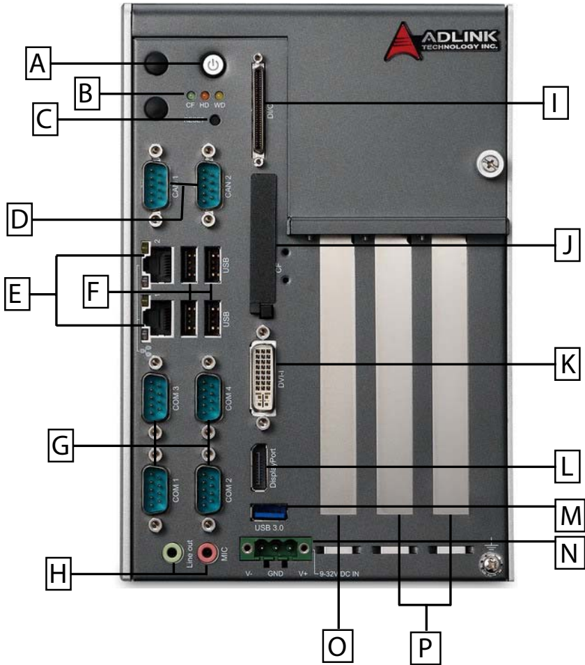
Figure 1-7: Front Panel I/O Connectors
