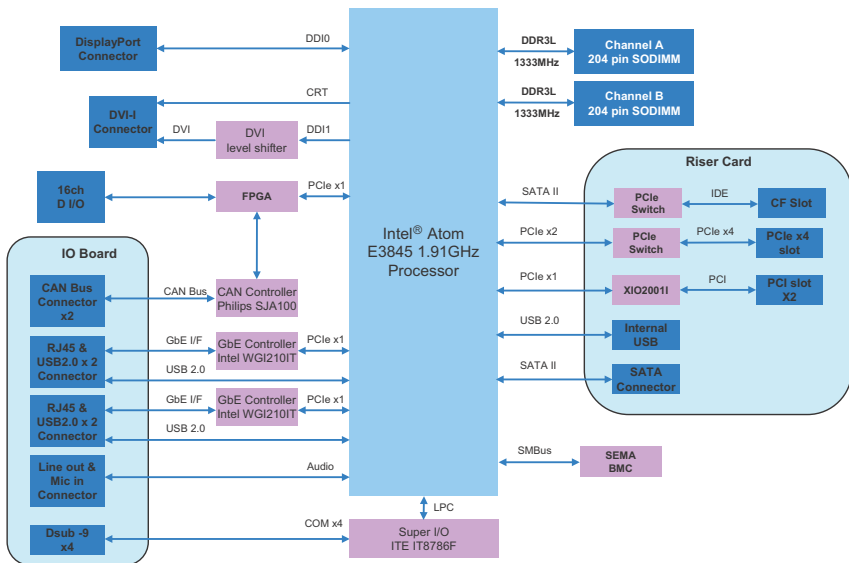
Figure 1-1: MXC-2300 Functional Block Diagram
