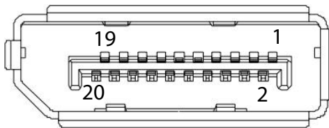
Figure 1-14: DisplayPort Connector
