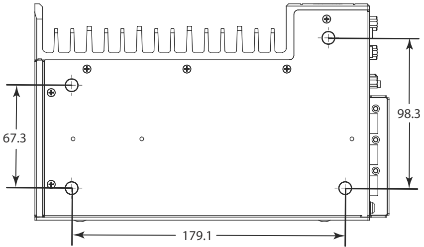
Figure 1-6: MXC-2300 Underside View
