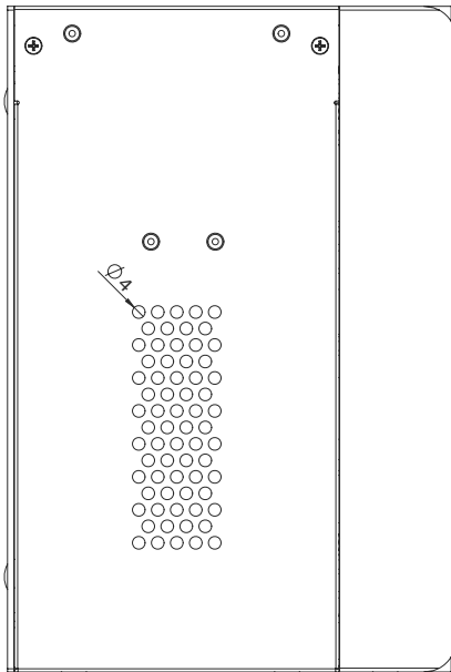
Figure 1-5: MXC-2300 Rear View
