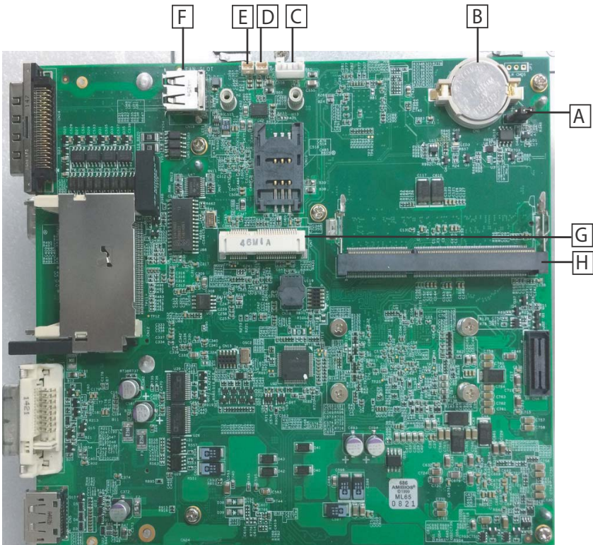
Figure 1-15: Mainboard PCB
