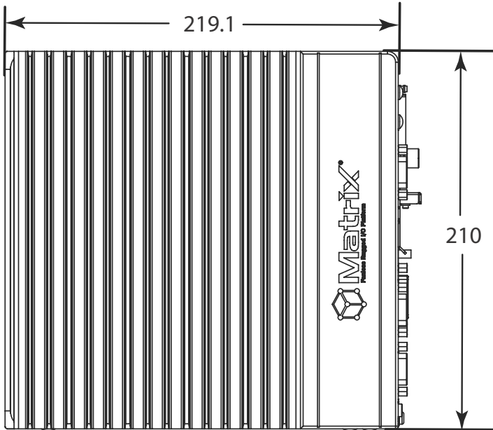
Figure 1-2: MXC-2300 Left Side View
